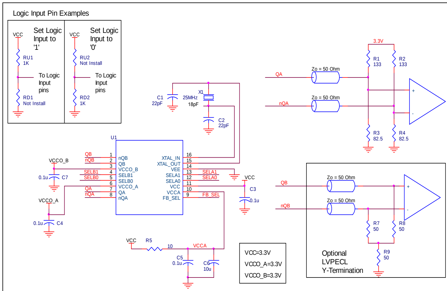
Figure 5. 843252 Schematic Example
