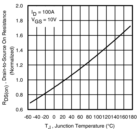
Fig 6. Normalized On-Resistance vs. Temperature
