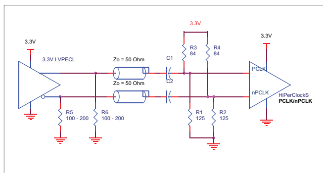
FIGURE 5D. PCLK/nPCLK INPUT DRIVEN BY A 3.3V LVPECL DRIVER WITH AC COUPLE
