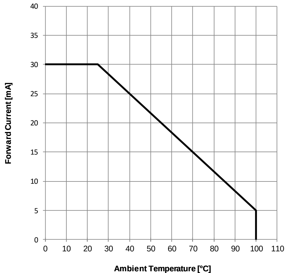
Derating Curve:
