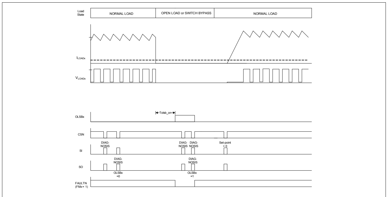
Figure 22 OLSB Fault - On State Timing Diagram (Low-Side Configuration)
