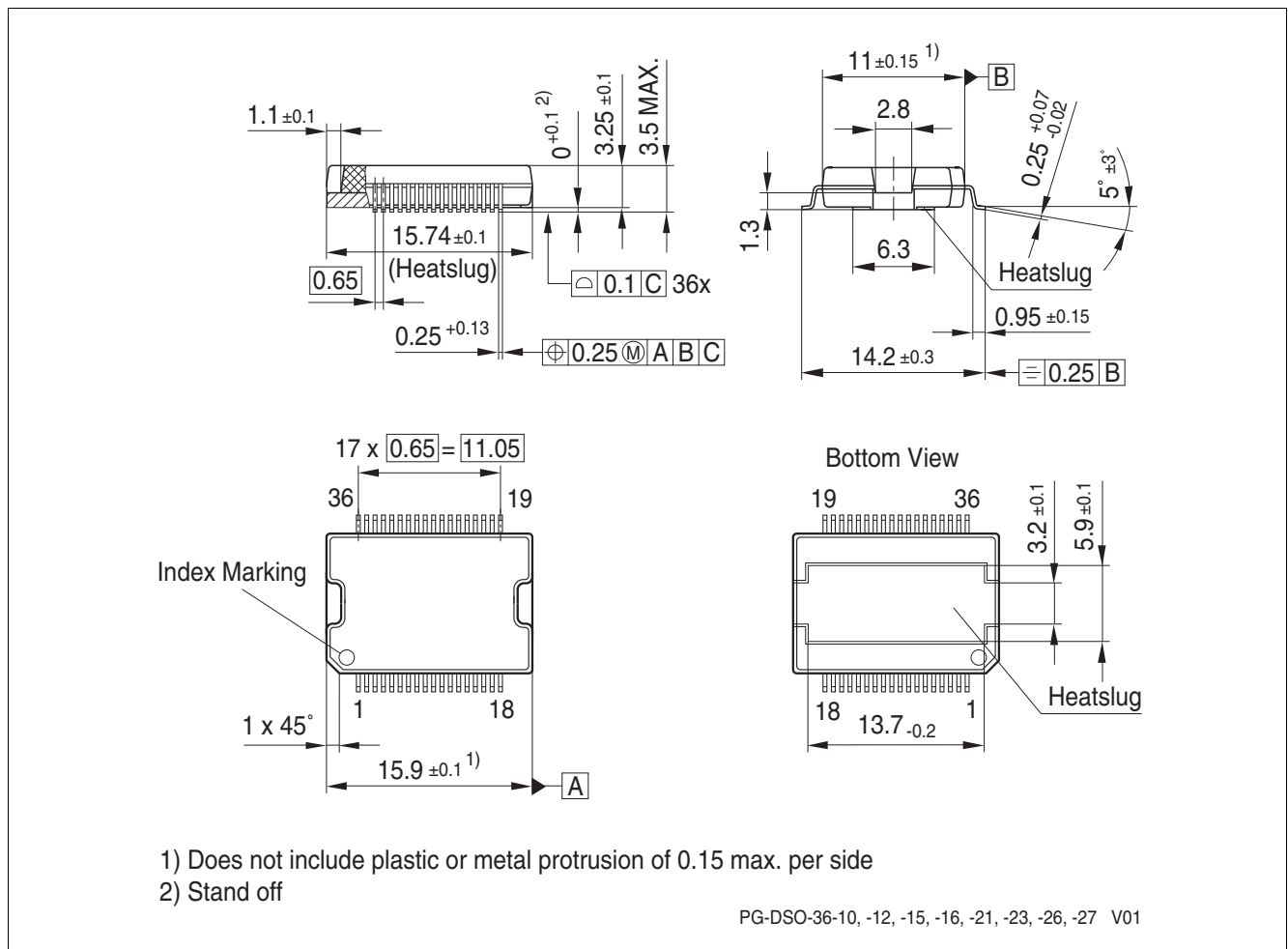
Figure 39 PG-DSO-36
