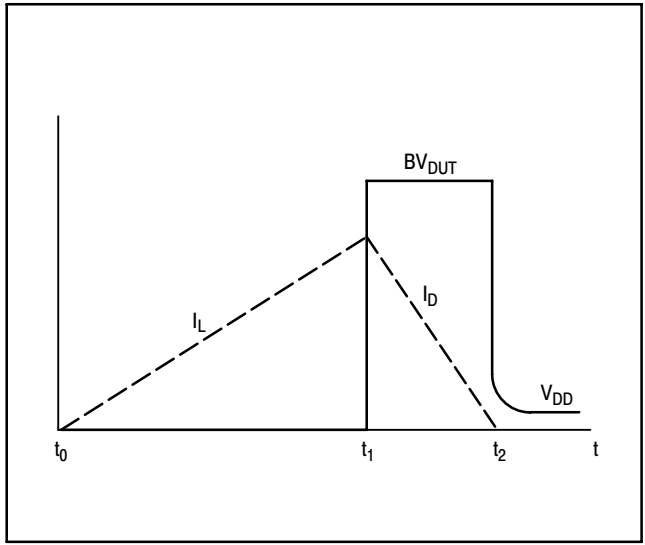
Figure 7. Current-Voltage Waveforms
