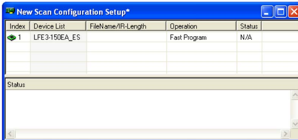
Figure 10. ispVM New Scan Configuration Setup
