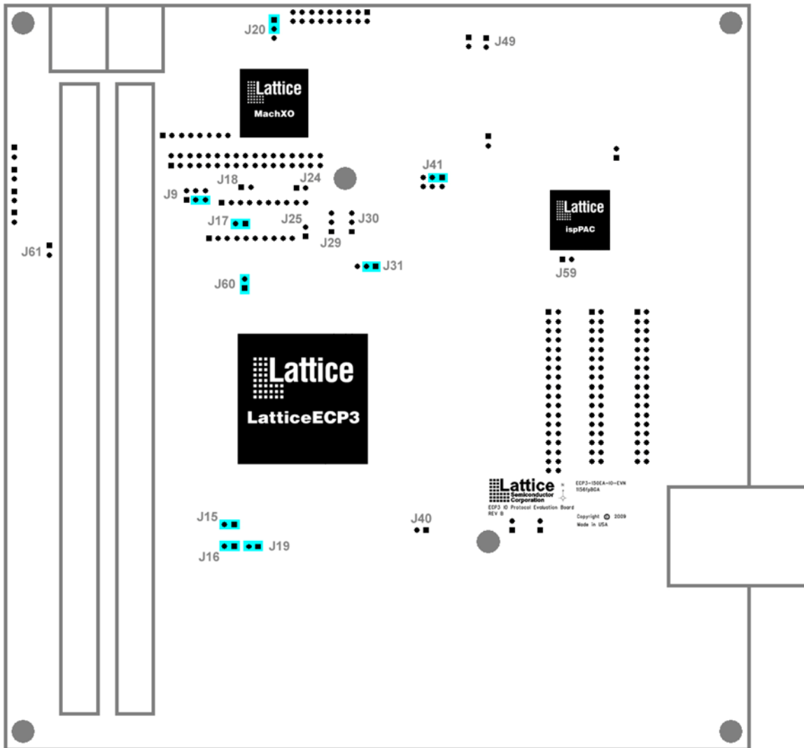
Figure 7. Default Jumper Settings
