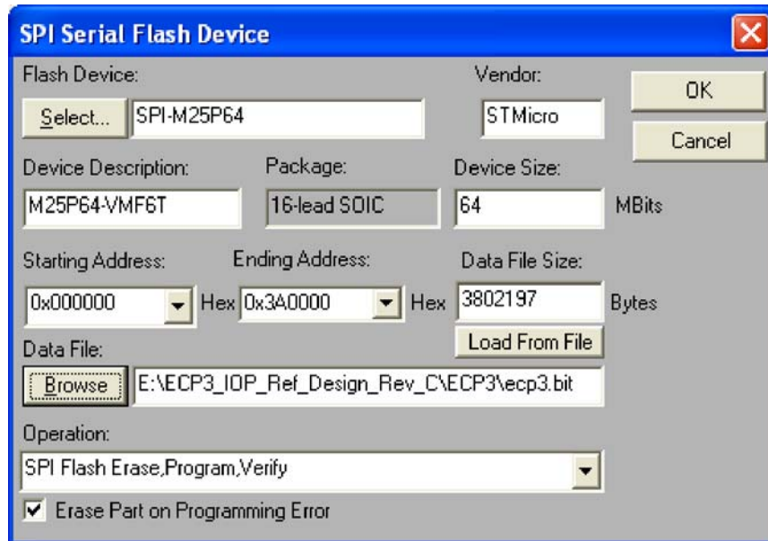
Figure 16. SPI Flash Device Setup Complete
