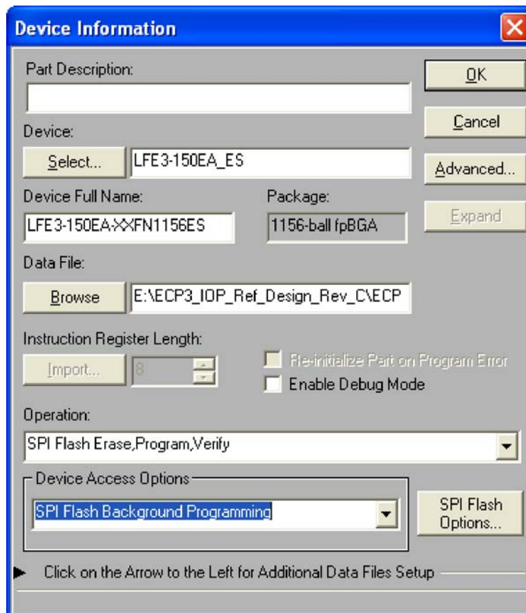
Figure 17. Bitstream Ready to Download into SPI Flash
