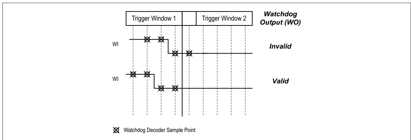
Figure 8 Valid triggering
