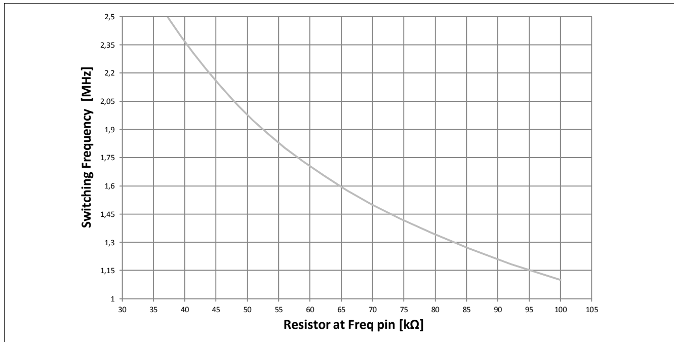
Figure 13 Switching frequency f_{\text{OSC}} versus frequency setting resistor R_{\text{FREQ}} .
