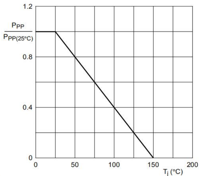
Fig 2. Relative variation of peak pulse power as a function of junction temperature
