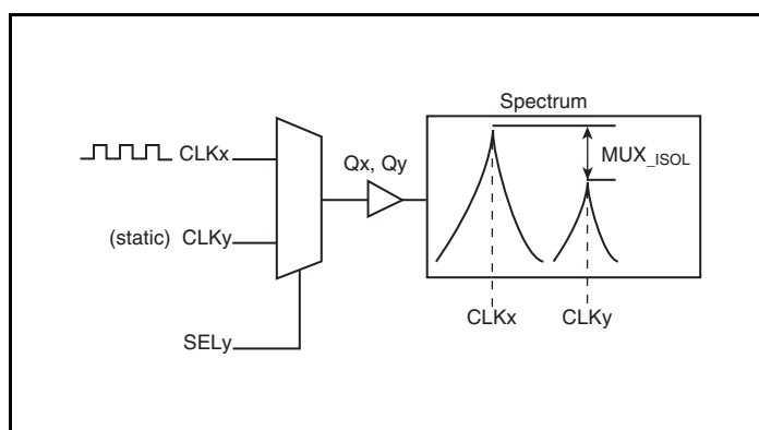
MUX Isolation
