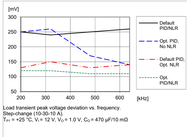
Load transient vs. Switch Frequency
