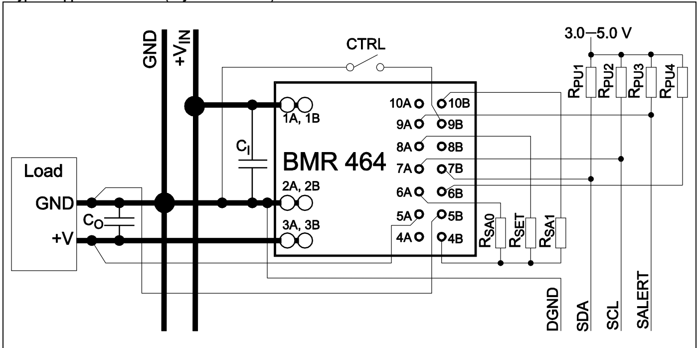
Typical Application Circuit (Lay Down version)
