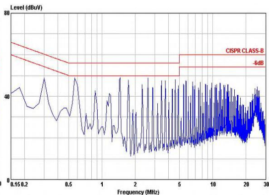
Conduction Emission of EN55022 Class B
