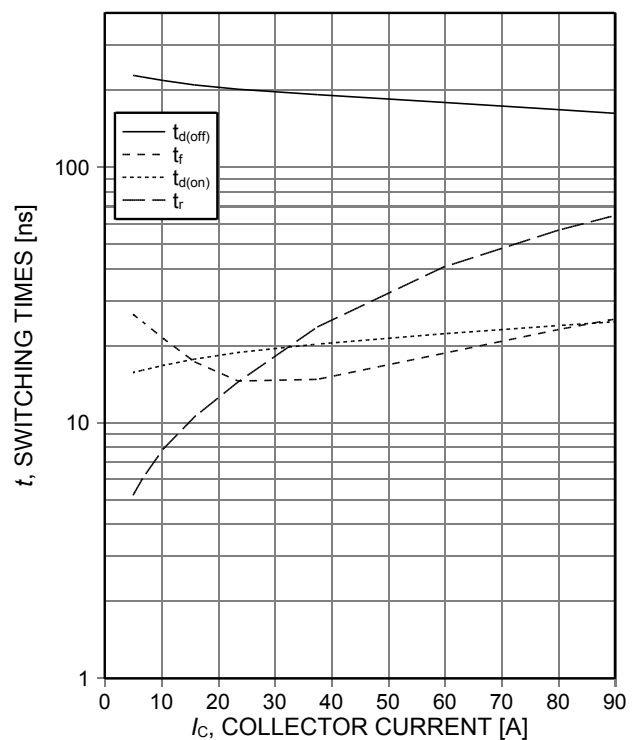
Figure 8. Typical switching times as a function of collector current (inductive load, T_j=150^{\circ}\text{C} , V_{CE}=400\text{V} , V_{GE}=15/0\text{V} , r_G=23\Omega , Dynamic test circuit in Figure E)
