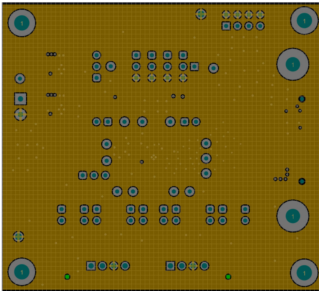
Figure 5-2. Power Plane 1
