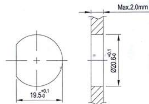
Panel cut-out
