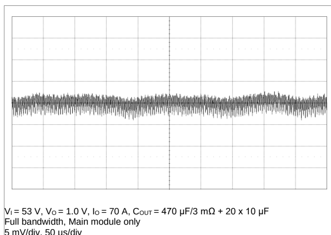
Example of low frequency ripple at the output.
