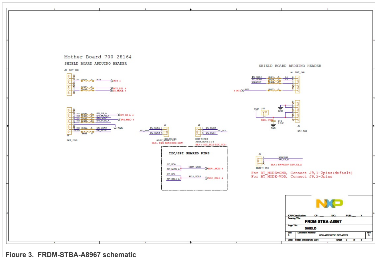
Figure 3. FRDM-STBA-A8967 schematic
