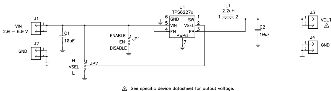
Figure 11. TPS6227XEVM-306 Schematic
