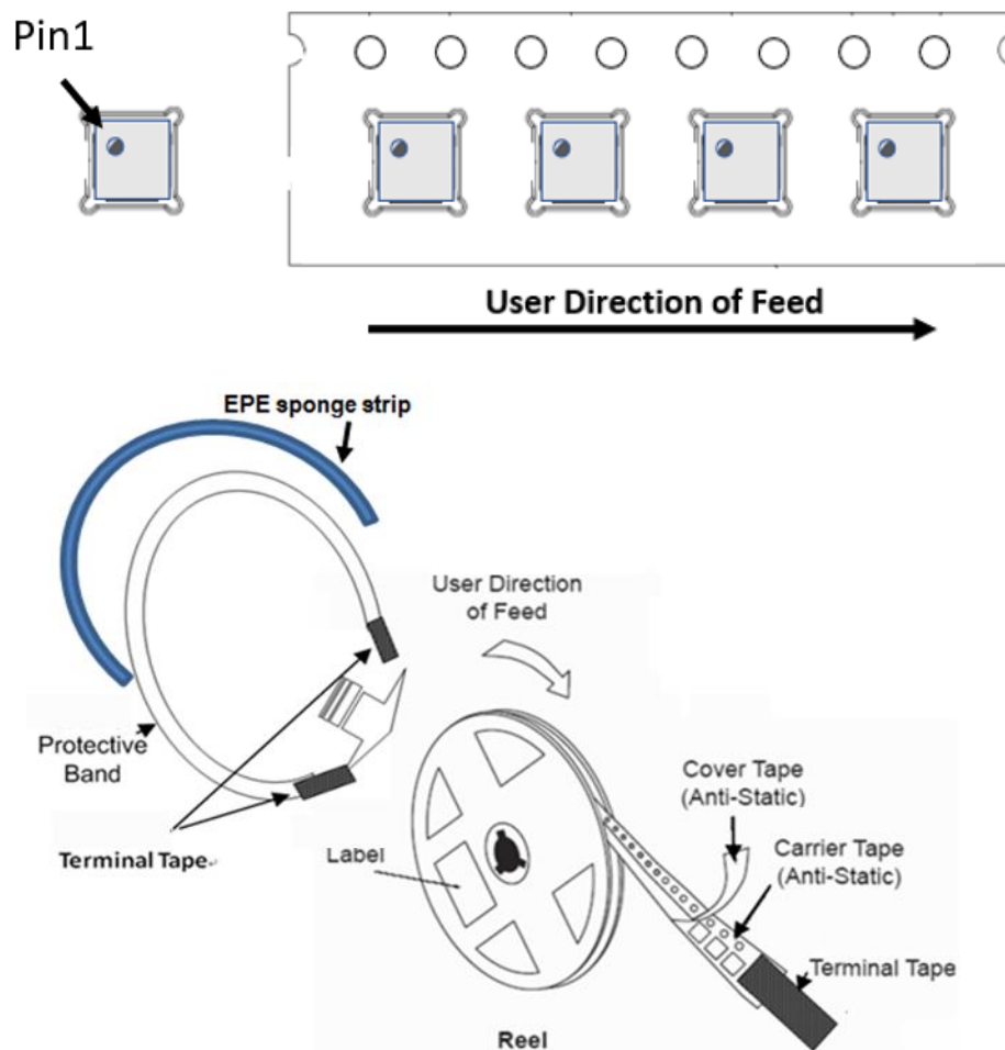
Figure 22. ICP-20100 Tape and Reel Drawing
