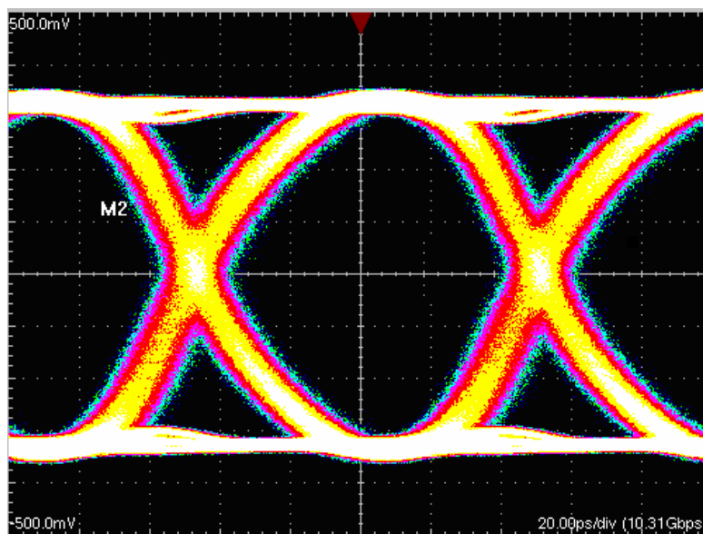
FIGURE 3. ISL36411 10.3125Gb/s OUTPUT FOR A 10M 28AWG CABLE
