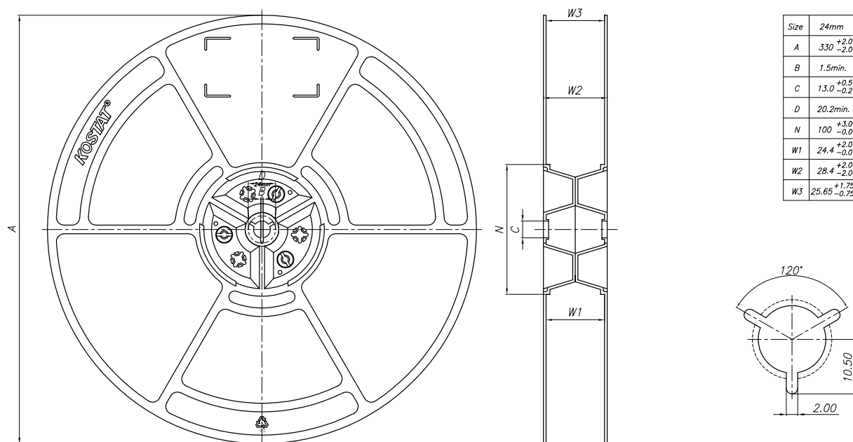
Figure 7. Plastic reel
