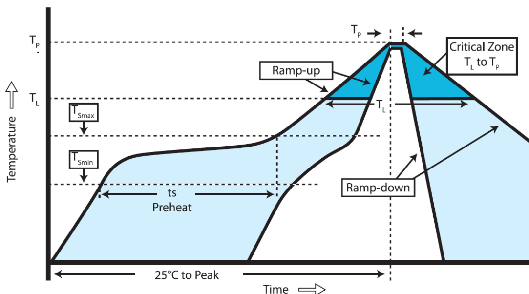
Figure 10. Soldering profiles
