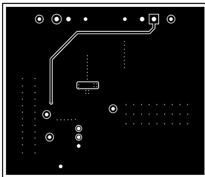
Figure 5-3. Bottom Layer
