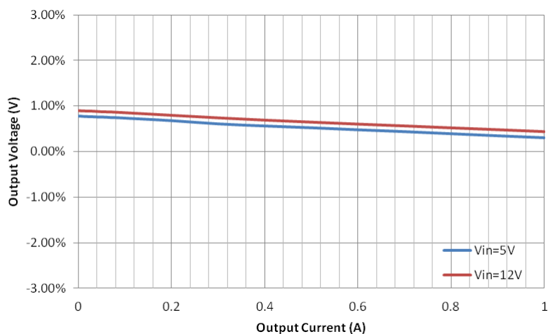
Figure 4-3. Load Regulation
