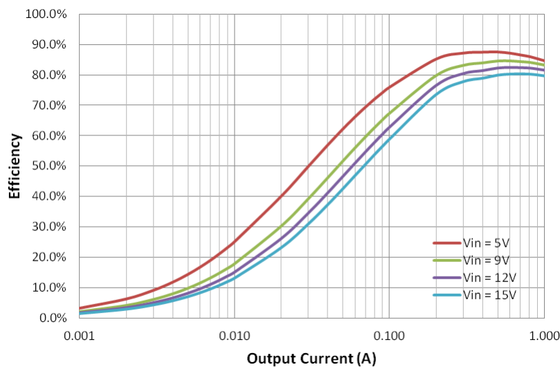
Figure 4-1. Efficiency
