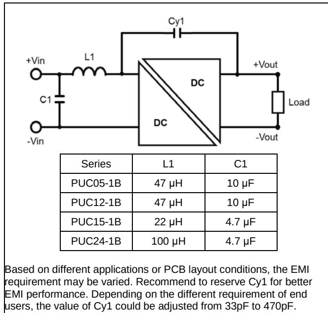
Test set-up
