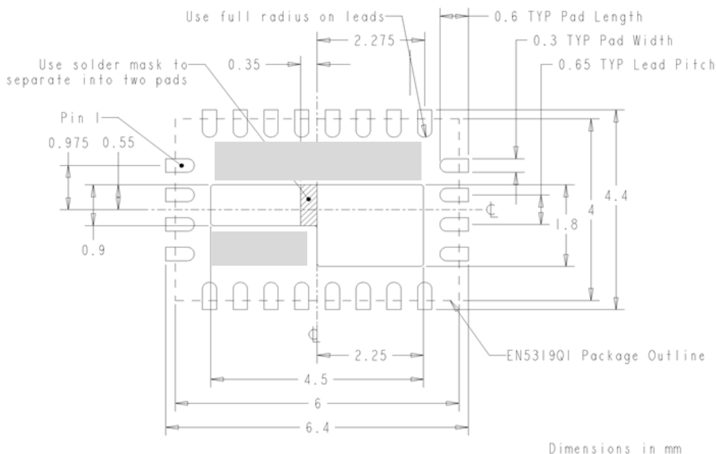
Figure 10: Lead-Frame exposed metal (Top View)
