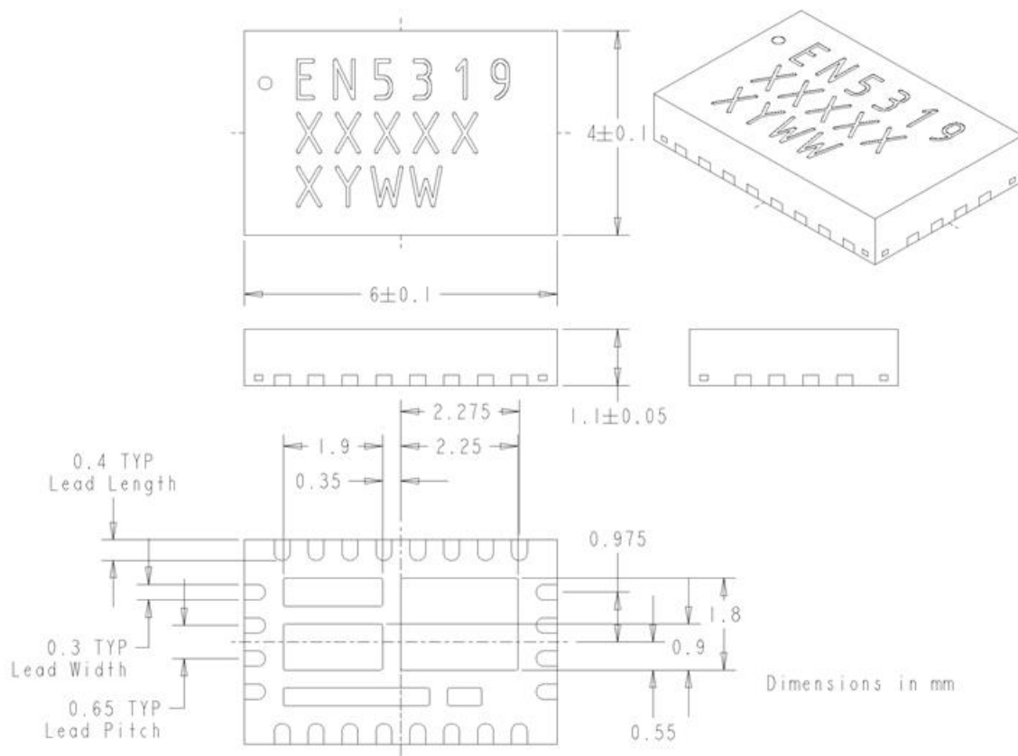
Figure 12: EN5319QI Package Dimensions (Bottom View)
