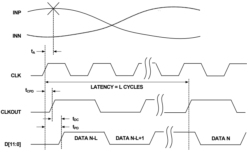
FIGURE 1A. LVDS
