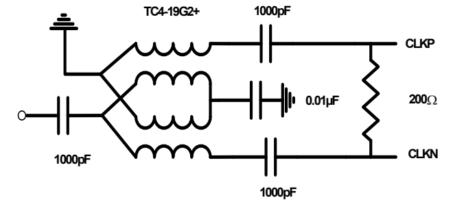
FIGURE 31. RECOMMENDED CLOCK DRIVE A selectable 2x frequency divider is provided in series with the clock input. The divider can be used in the 2x mode with a sample clock equal to twice the desired sample rate. This allows the use of the Phase Slip feature, which enables synchronization of multiple ADCs. The Phase Slip feature can be used as an alternative to using the CLKDIVRST pins to synchronize ADCs in a multiple ADC system.
