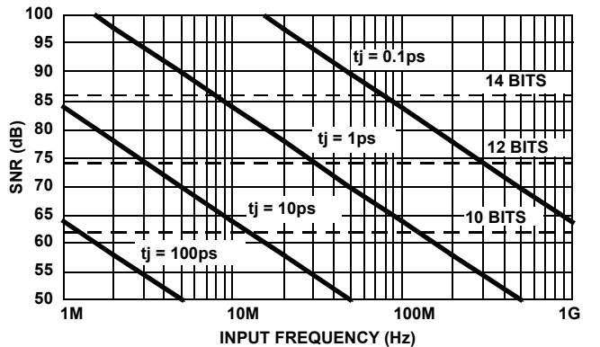
FIGURE 32. SNR vs CLOCK JITTER This relationship shows the SNR that would be achieved if clock jitter were the only non-ideal factor. In reality, achievable SNR is limited by internal factors such as linearity, aperture jitter and thermal noise. Internal aperture jitter is the uncertainty in the sampling instant shown in Figure 1A. The internal aperture jitter combines with the input clock jitter in a root-sum-square fashion, since they are not statistically correlated, and this determines the total jitter in the system. The total jitter, combined with other noise sources, then determines the achievable SNR.
