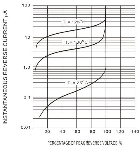
Fig.3-TYPICAL REVERSE CHARACTERISTIC
