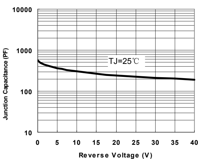
Fig.1-Typical Junction Capacitance
