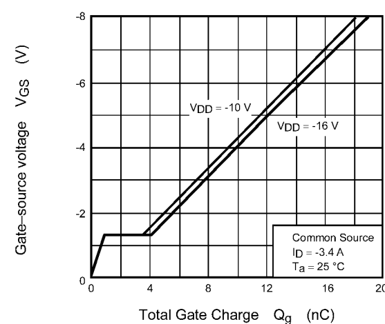
Fig. 8.12 Dynamic Input Characteristics
