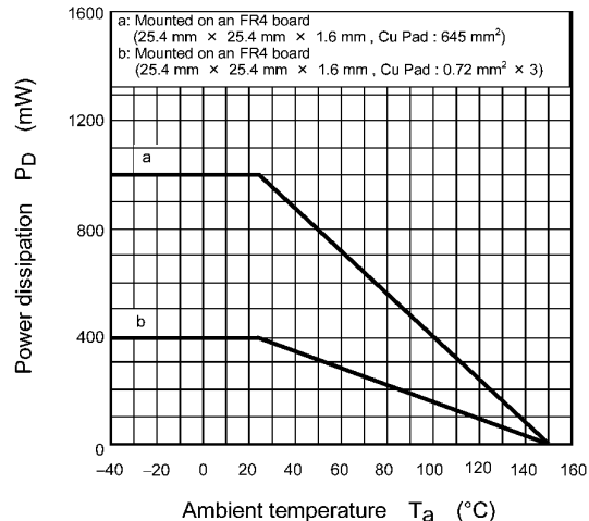
Fig. 8.14 P_D - T_a
