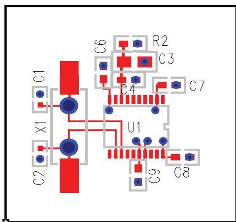
FIGURE 4B. 843002-01 PC BOARD LAYOUT EXAMPLE
