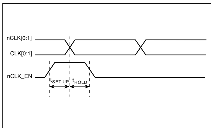
Setup & Hold Time
