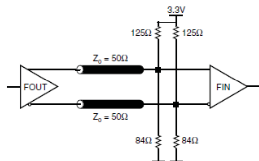
FIGURE 4B. LVPECL OUTPUT TERMINATION
