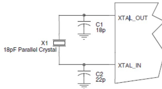
Figure 3. CRYSTAL INPUT INTERFACE
