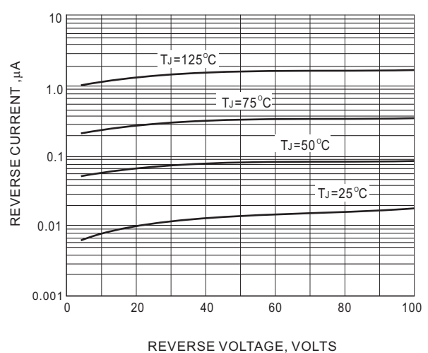
FIG. 2-TYPICAL REVERSE CHARACTERISTICS
