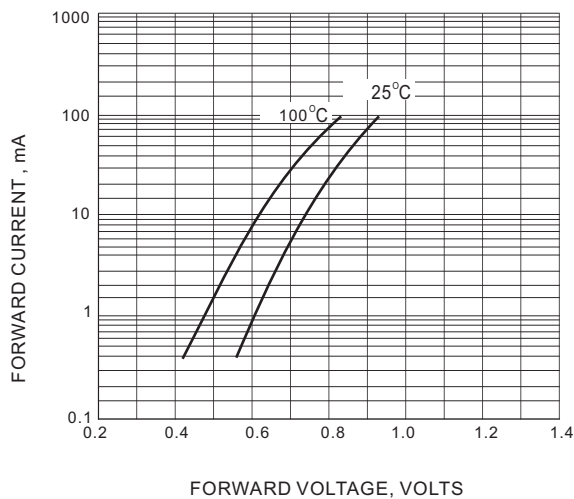
FIG. 1-TYPICAL FORWARD CHARACTERISTIC
