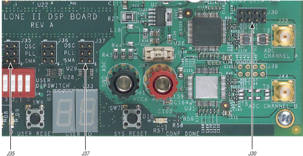
Figure 2–8. Locations of Jumpers J30, J35 & J37
