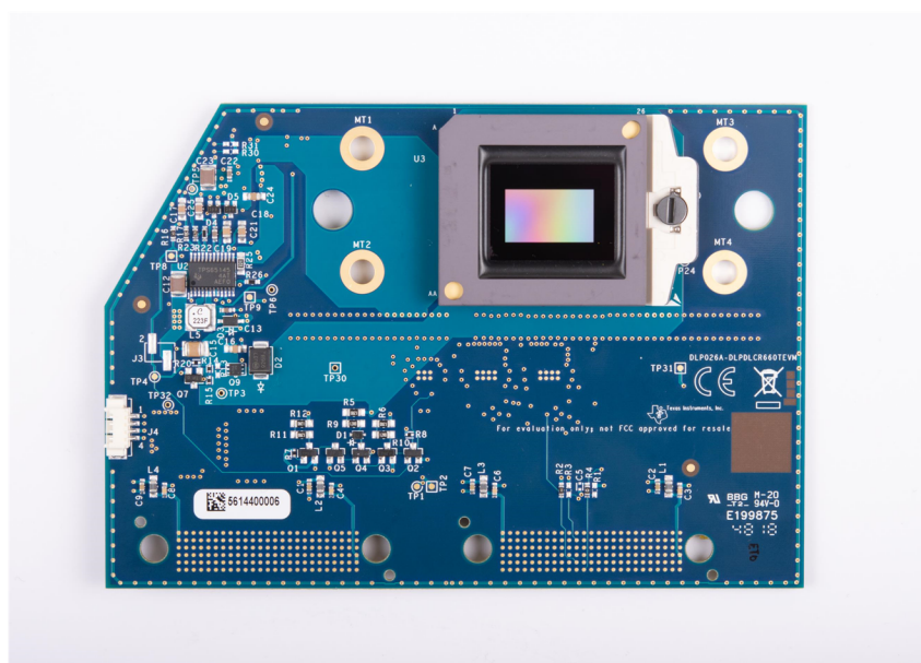
Figure 1-2. DLPDLCR660TEVM
