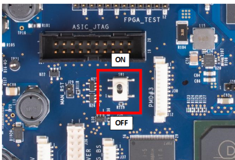
Figure 2-4. ON/OFF Switch
