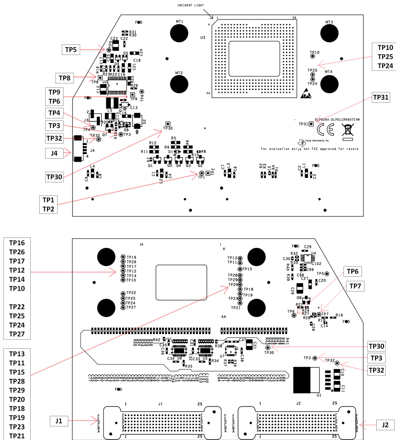
Figure 3-2. DLPDLCR660TEVM Test Points and Connectors
