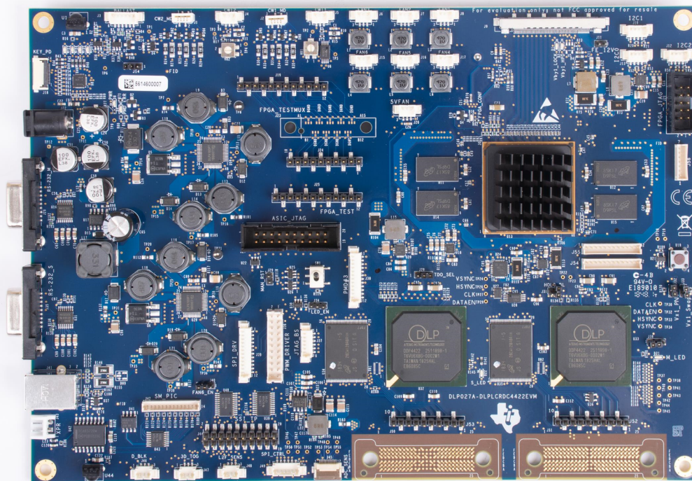
Figure 1-1. DLPLCRDC4422EVM
