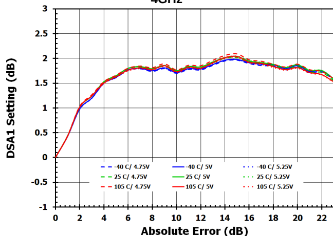
Figure 57. DSA1 Absolute Attenuation Error (INL) at 4GHz
