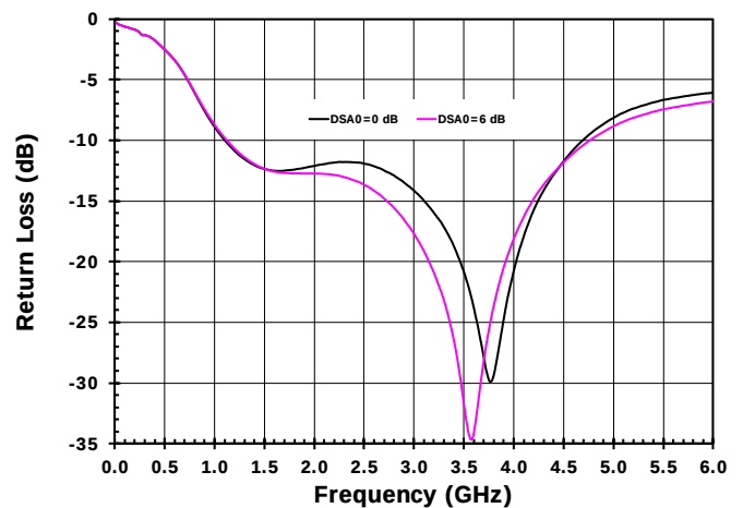
Figure 9. Output Return Loss for DSA0 Settings
