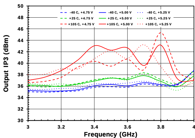
Figure 30. OIP3 vs. Frequency with P_{OUT} = 0\text{dBm/Tone} and DSA0 = 6\text{dB}
