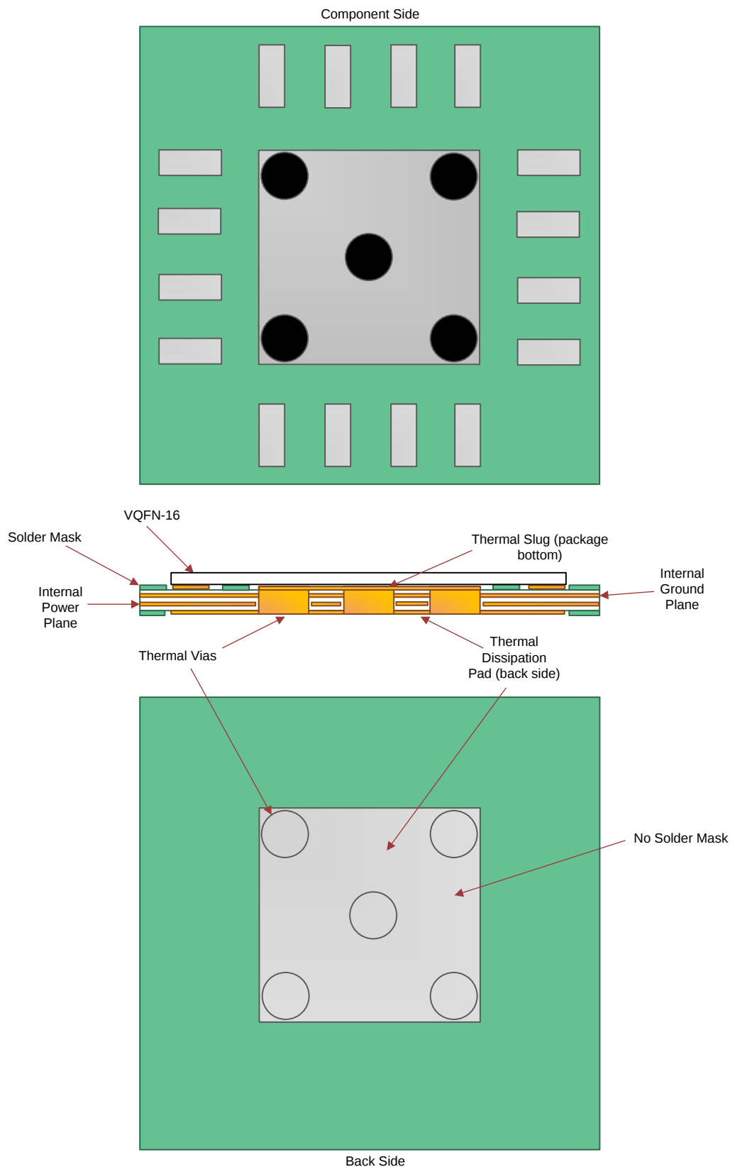
Figure 6. Layout Example
