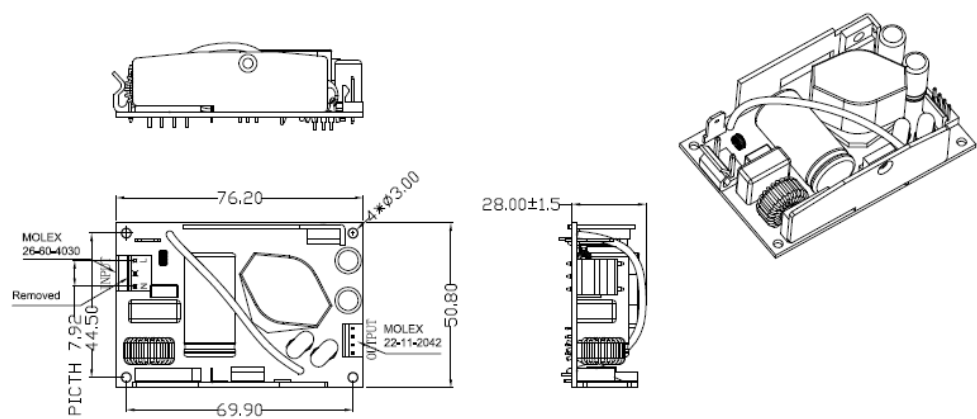
Alternative configuration for F2 grounding
