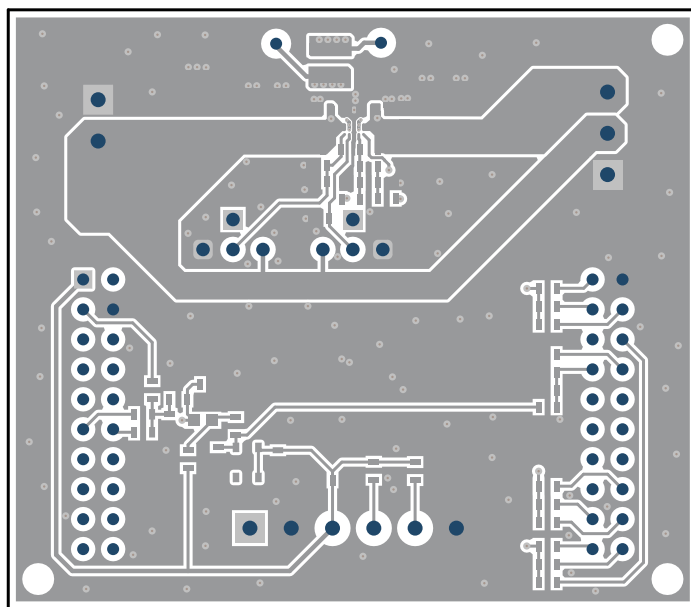
Figure 8-2. Top Layer
