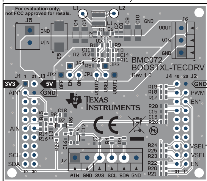
Figure 8-1. Assembly Layer
