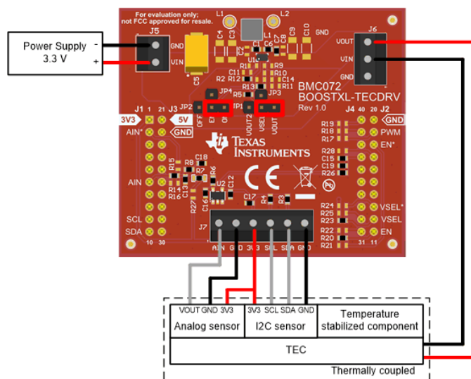
Figure 7-1. Hardware Setup
