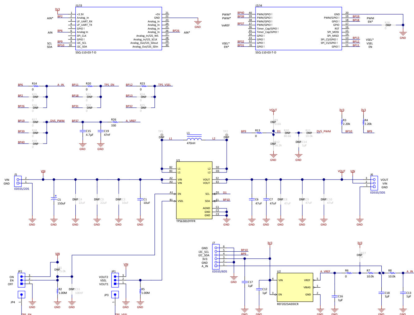
Figure 8-4. BOOSTXL-TECDRV Schematic
