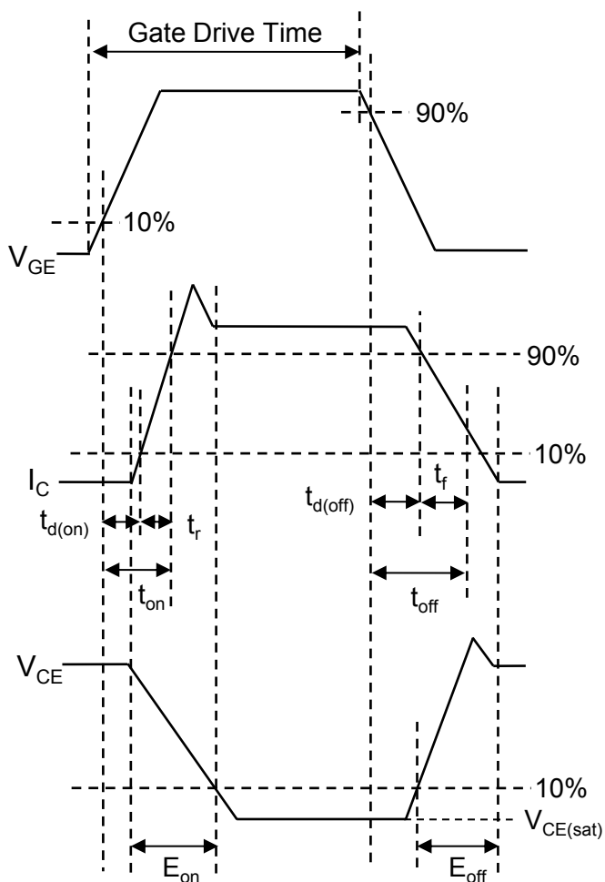
Fig.24 Inductive Load Waveform
