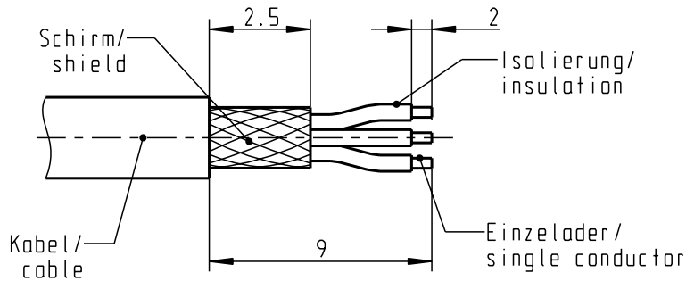
empfohlene Abisolierlänge/ recommended Cable Preparation
