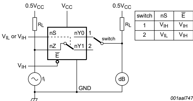
Fig. 19. Test circuit for measuring isolation (OFF-state)
