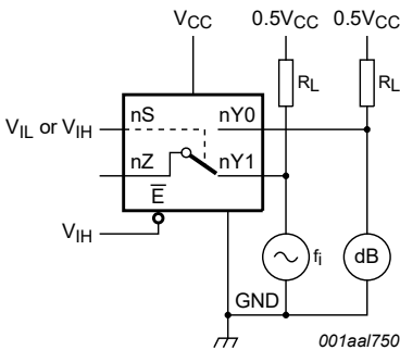
Fig. 21. Test circuit for measuring crosstalk between switches
