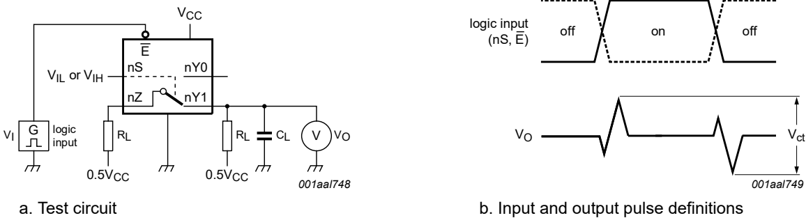
Fig. 20. Test circuit for measuring crosstalk voltage between digital inputs and switch
