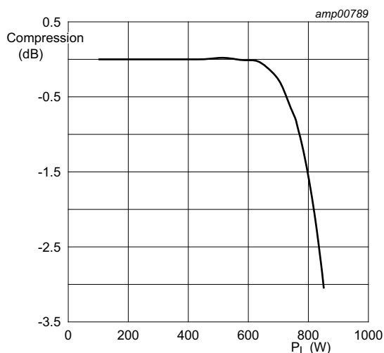
Fig 3. Compression as a function of output power; typical values
