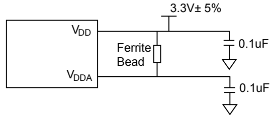
Figure 12. Power Supply Filter
