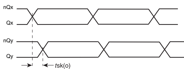
Figure 6. Output Skew
