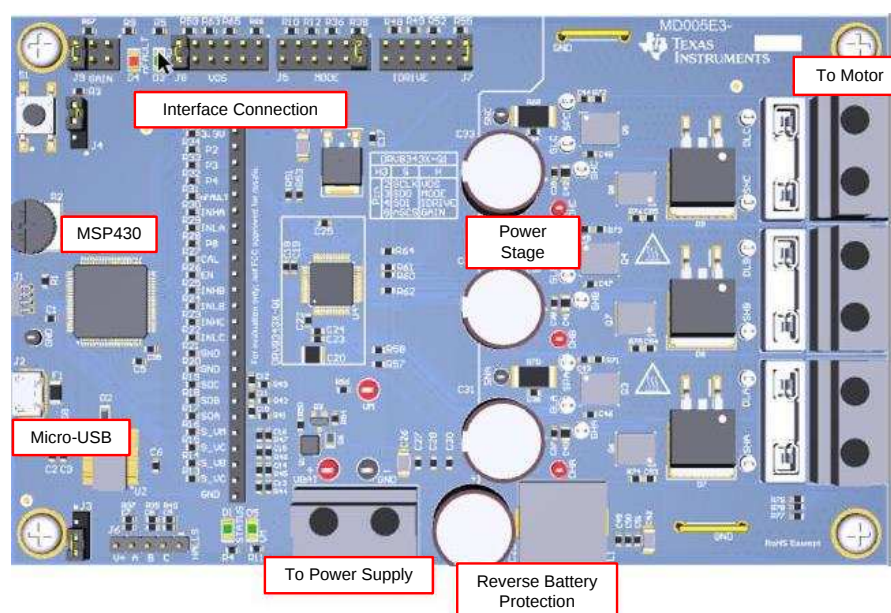
Figure 1. DRV8343x-Q1EVM Top View
