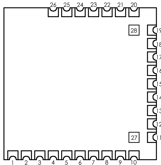
Figure 2 - BMD-200 Pin-out
