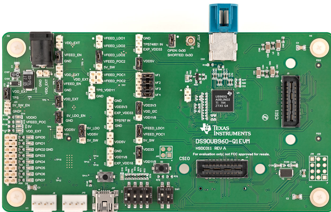
Figure 1-1. DS90UB960-Q1EVM
