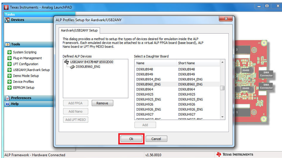
Figure 9-4. Finish Setup
