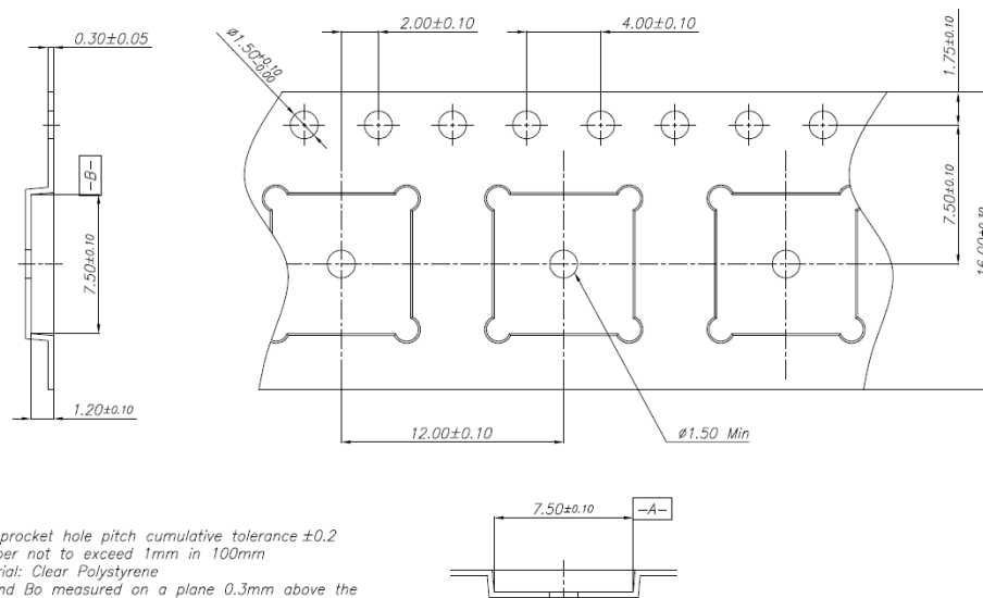
Figure 5: Orientation of EVA-8M modules on the tape
