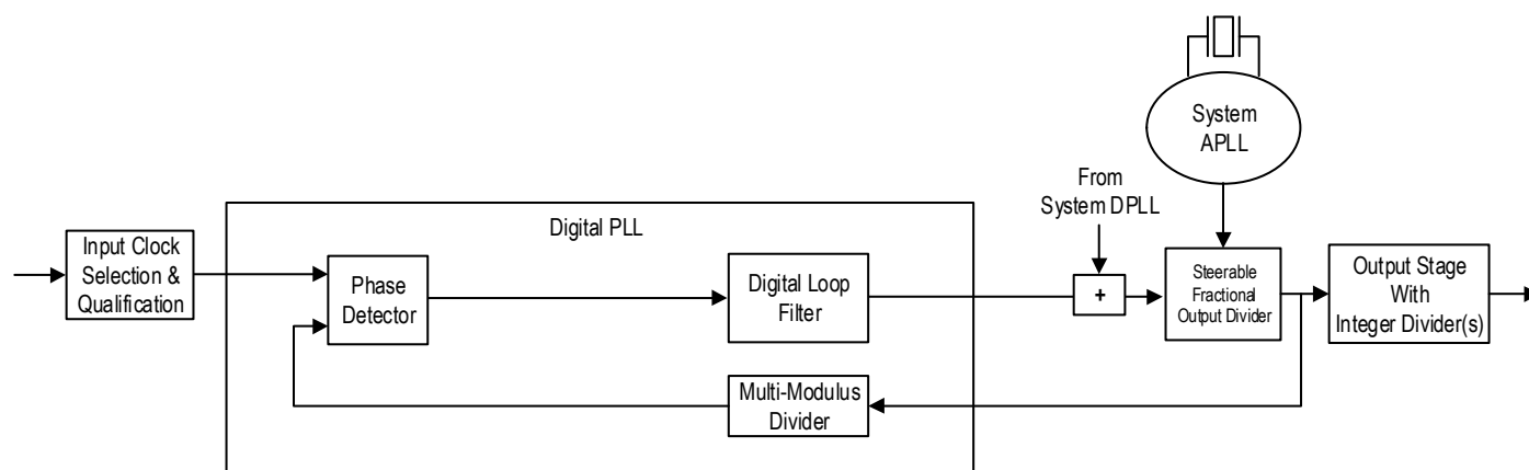
Figure 28. Jitter Attenuator Disciplined with Oscillator Operation
