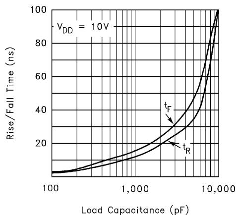
FIGURE 9. RISE/FALL TIME vs LOAD
