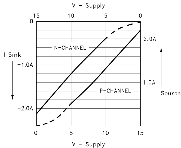
FIGURE 4. PEAK DRIVE vs SUPPLY VOLTAGE
