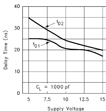
FIGURE 11. PROPAGATION DELAY vs SUPPLY VOLTAGE
