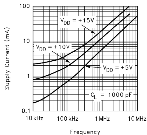
FIGURE 7. AVERAGE SUPPLY CURRENT vs VOLTAGE AND FREQUENCY
